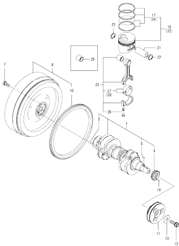
Fig.7. CRANKSHAFT & PISTON
