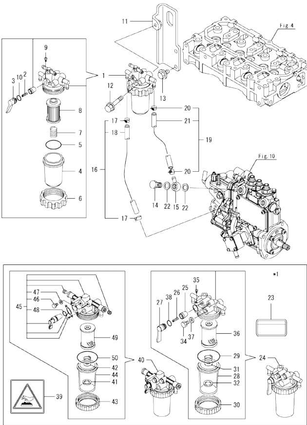
Fig.13. FUEL PIPE
